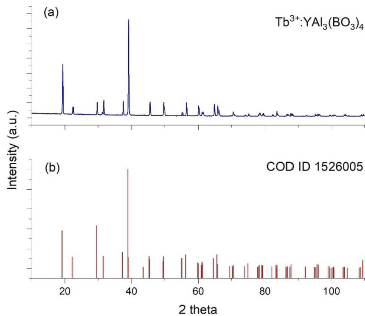
Fig. 2. XRPD patterns of (a) Tb:YAl 3 (BO 3 ) 4 crystal and (b) calculated from YAl 3 (BO 3 ) 4 cif-file (Crystallography open database ID 1526005)
