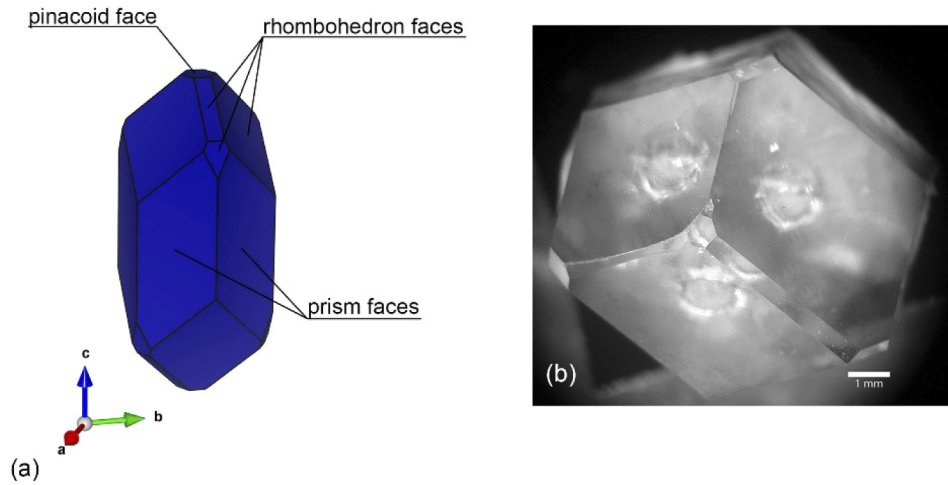
Fig. 1. (a) the growth habit of Tb:YAl 3 (BO 3 ) 4 crystal (visualization: VESTA [16]) and (b) the image of crystal head
